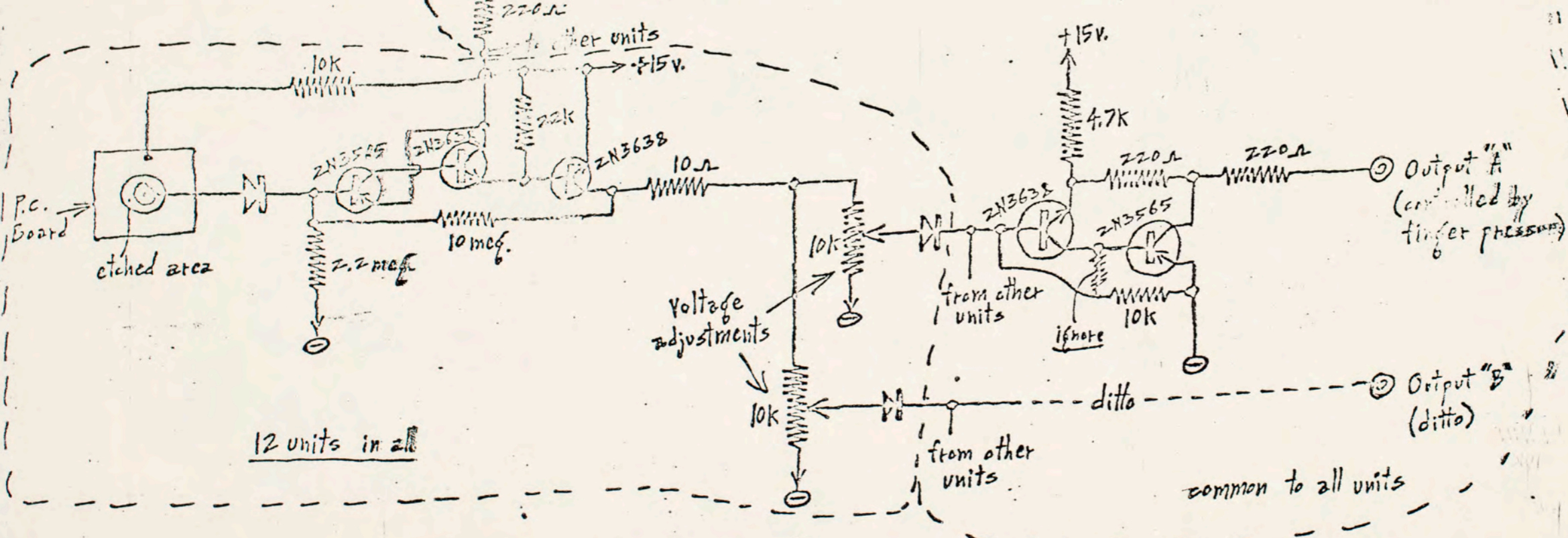
Buchla Touch-controlled Voltage Source (model 112)
