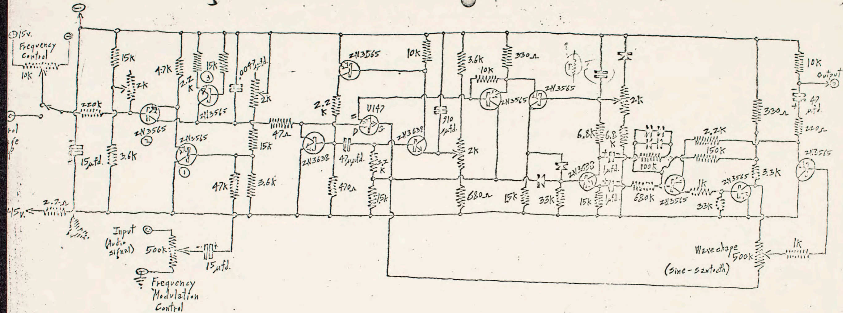
1/2 Buchla Dual Sine-sawtooth Generator (Model 158)
